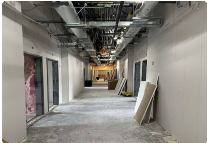
Second floor corridor showing drywall installation progress.
